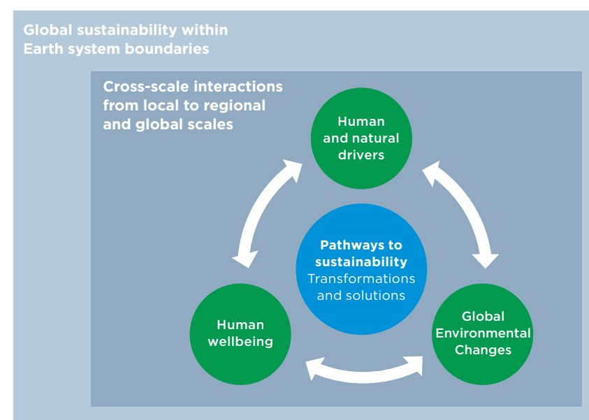
Figure 1: Schematics of the Future Earth conceptual framework
