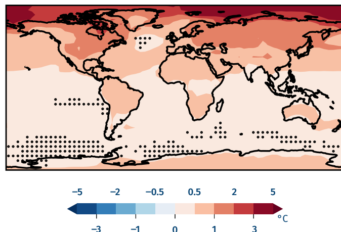
Figure 7. Five-year temperature forecasts. Ensemble mean predictions for near-surface temperature anomalies relative to 1991–2020 for the next five extended seasons of May to September 2024–2028 (left) and November to March 2024/2025–2028/2029 (right). Stippled where more than one third of models disagree on the sign of the anomaly. Source: WMO, 2024c
